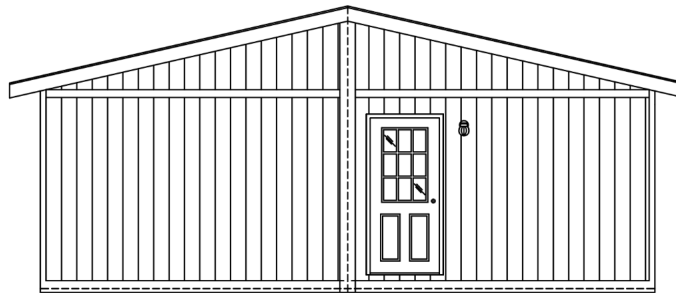
FRONT ENDWALL
